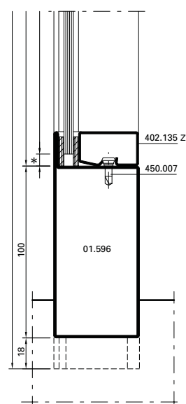
Detail E
